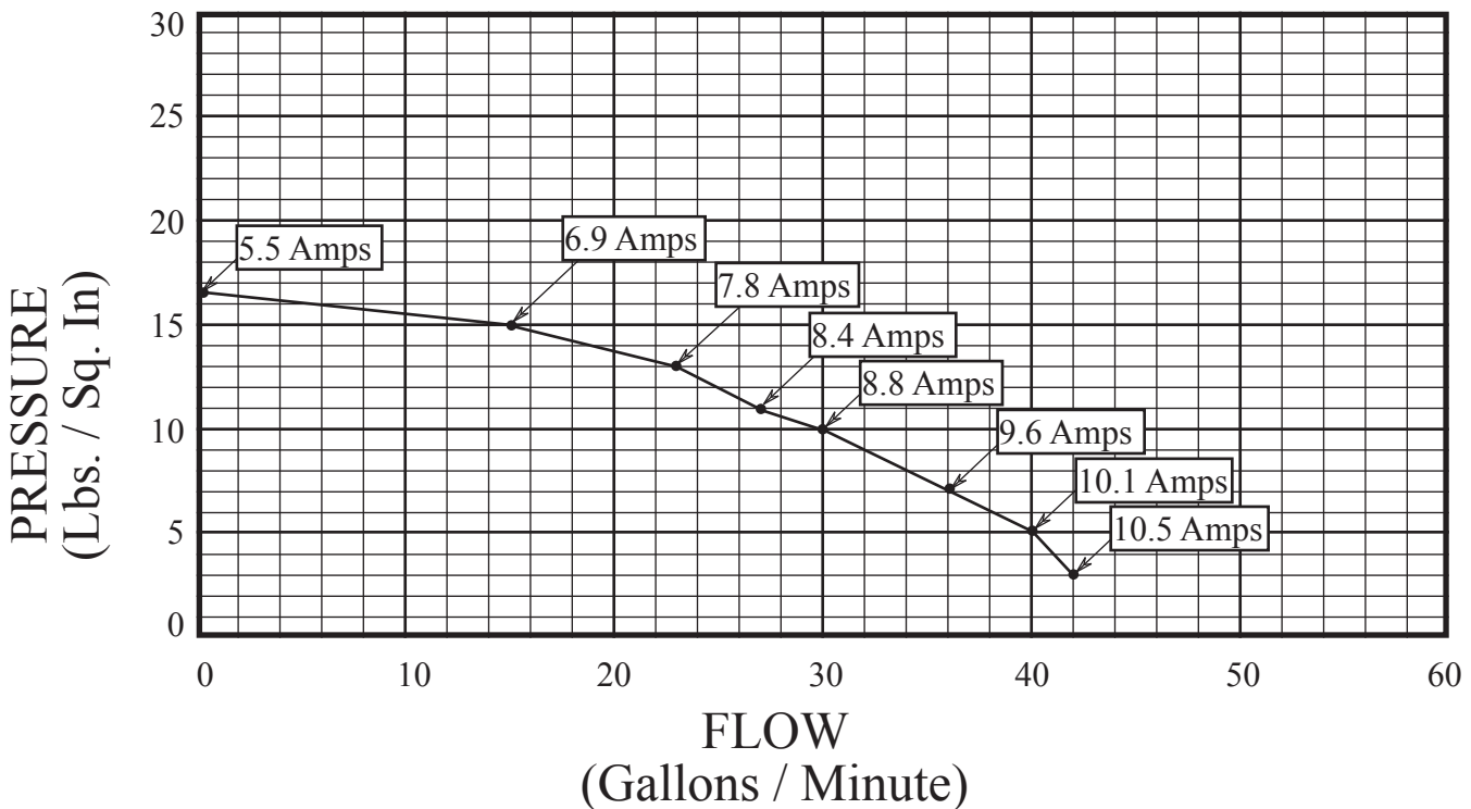
PUMP FLOW VS. PRESSURE @ 14VOLTS & 3200 RPM
